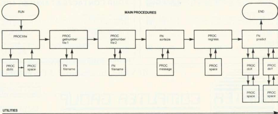
UTILITIES INCLUDED Figure 6. Structure of 'line of best fit' program
