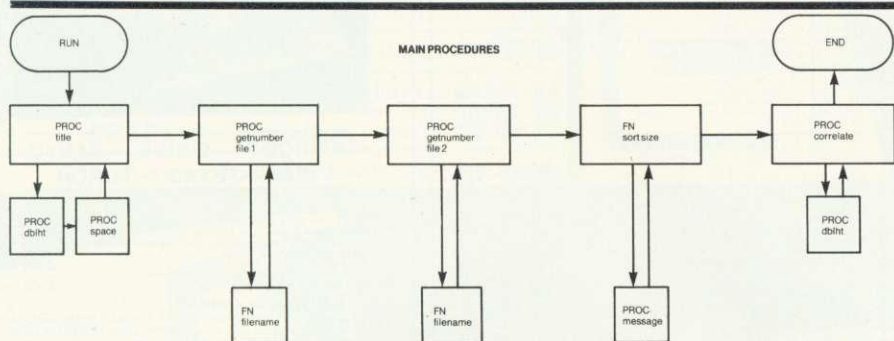
UTILITIES INCLUDED Figure 4. Structure of correlation program
